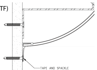
CLC-1 PF Perpendicular Fin
