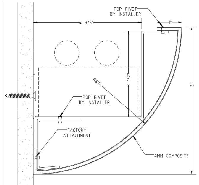
CLC-1 WM Wall Mount
